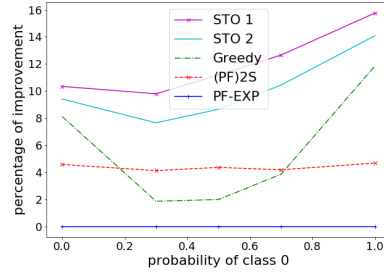
Fig. 8. Percentage improvement over PF-EXP. Heterogeneous velocities. p = 2/9 .
