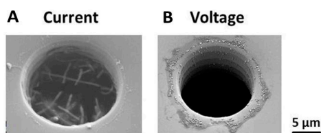
Figure 6. Different morphologies for gold deposition according to (A) current or (B) voltage applications in the CLEF protocol.
