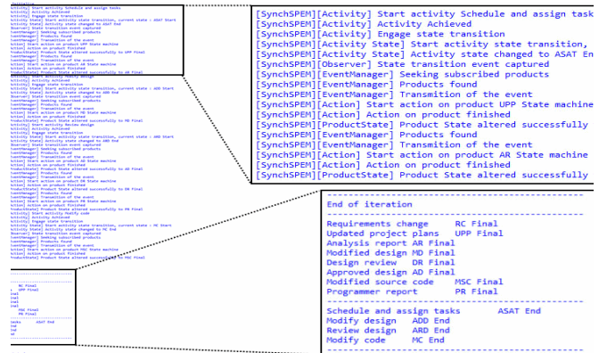
Figure 8. The execution trace.
