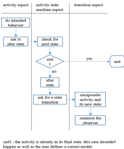
Figure 6. Lifecycle of an activity state change.
