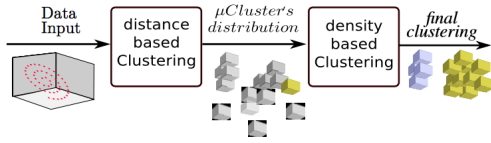
Figure 1: Overview of DyClee
