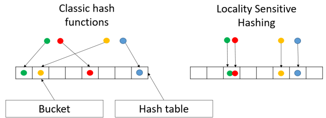
Figure 2: Assignment of samples with hash functions with the LSH
