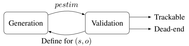
Figure 3: Algorithm structure.
