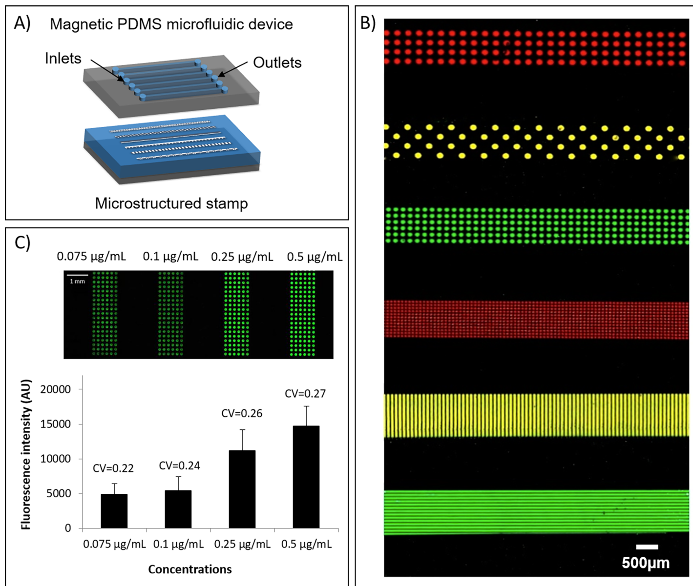
Fig 4. Multiplexed protein patterning. (A) Representative scheme of the fluidic cartridge and the structured stamp for multiplexed fluidic inking. (B) Fluorescence image of multiplexed protein deposition of Cy3-labeled streptavidin (green), Cy5-labeled streptavidin (red) and a mix of both previous solutions (yellow). Patterns dimensions were ranging from 50 \mu\text{m} to 150 \mu\text{m} . The image was obtained by fluorescence scanner InnoScan1100AL (PMT 532nm: 100%, PMT 635nm: 100%, Brightness: 10%, Contrast: 70%, Balance: 44%, resolution 3 \mu\text{m}/\text{pixel} ). (C) Fluorescence image after multiplexed fluidic inking and one-step printing of Cy3-labeled streptavidin with different inks of concentrations ranging from 0.075 \mu\text{g/mL} to 0.5 \mu\text{g/mL} .
