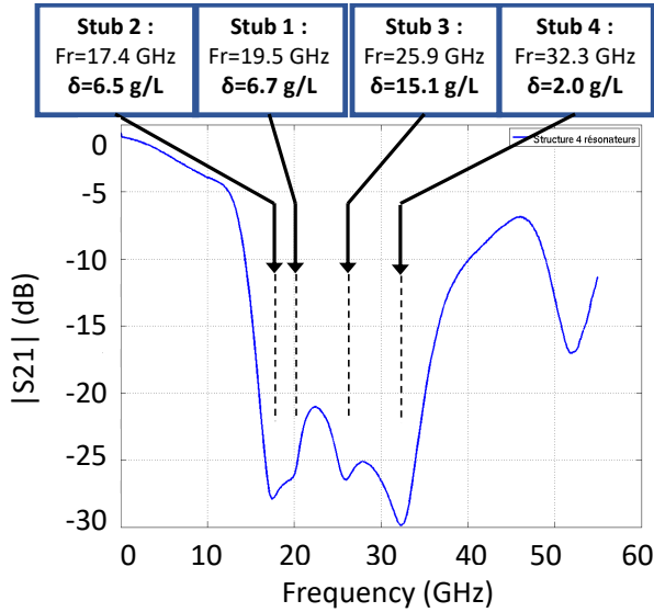
Fig. 2. Transmission coefficient of the quadruple stub sensor while empty.
