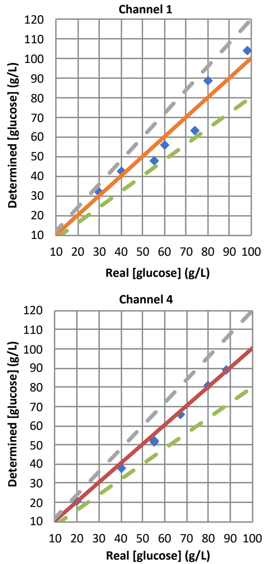
Fig. 3. Accuracy evaluation of glucose concentration in the Clark chart for channels 1 and 4.
