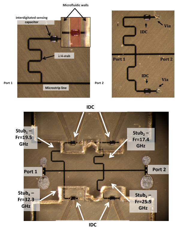
Fig. 1. Photographies of the single, double and quadruple interdigitated capacitor-based microwave biosensors.
