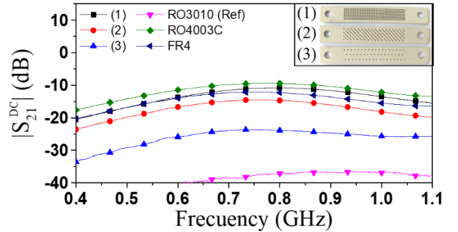
Fig. 4. Cross-mode transmission coefficient that results by loading the REF and the SUT lines with different solid samples.
