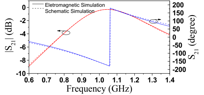
Fig. 2. Transmission coefficient (magnitude and phase) of the sensor (one half) inferred from circuit and electromagnetic simulation. The considered substrate is Rogers RO4003C with dielectric constant \epsilon_r = 3.38 , thickness h = 1.524 mm, and loss tangent \tan\delta = 0.0027 . In reference to Fig. 1, dimensions are: l = 40 mm, w = 3.4 mm, h = 9.4 mm, c = 0.2 mm, d = 2 mm, l_{ext} = 18.4 mm, h_{ext} = 3 mm, l_{int} = 13.4 mm, h_{int} = 1.4 mm, l_w = 44 mm and h_w = 26.8 mm. Circuit parameters are: L = 32.6 nH, C = 0.714 pF, G = 0.079 mS; line parameters are \beta l = 83^\circ and Z_0 = 50 \Omega .
