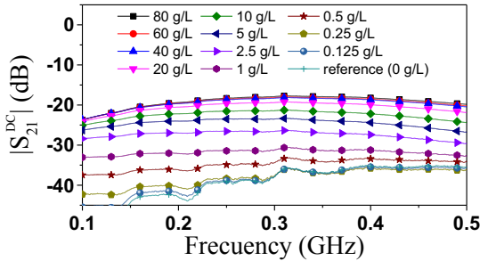
Fig. 6. Cross-mode transmission coefficient for different NaCl concentrations.
