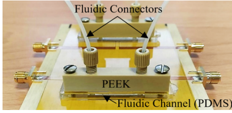
Fig. 5. Photograph of the sensor including fluidic channels and accessories. The fluidic channels, made of polydimethylsiloxane (PDMS), have dimensions: 26 mm (length), 4.6 mm (width), 1.5 mm (height). Such channels are covered by polyether ether ketone (PEEK) to provide mechanical stability.
