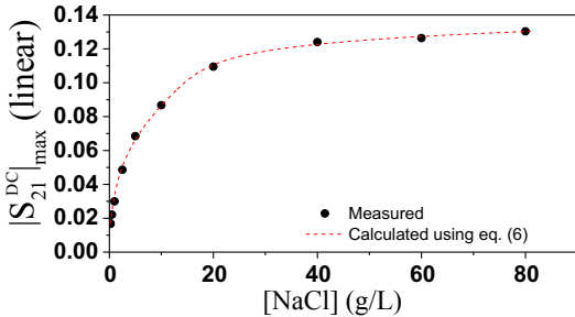
Fig. 7. Maximum cross-mode transmission coefficient with NaCl content.
