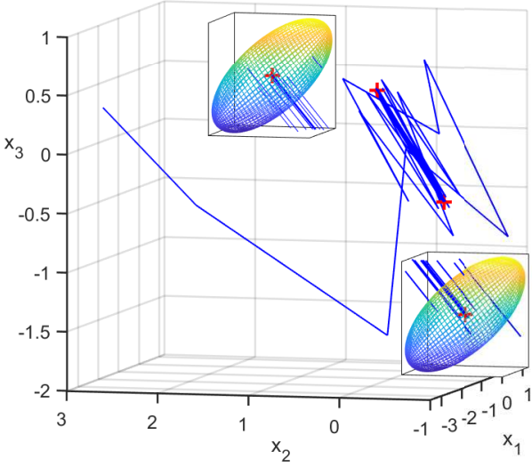
Fig. 1. Trajectories of system (1) for Example 1 in the state space. Two windows are included to show the attractor located around the shifted centers, represented by the red cross.
