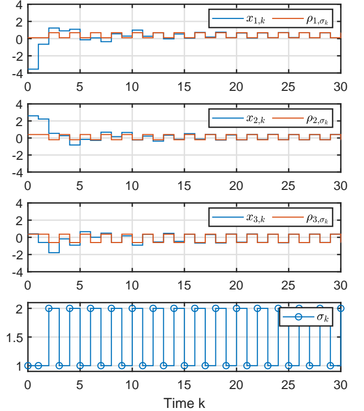
Fig. 2. Evolution of x_k - \rho_{\sigma_k} with the switching function \sigma \in \{1, 2\} computed at instant k
