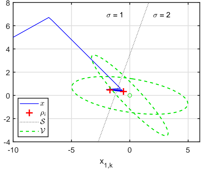
Fig. 5. Trajectories of system (1) for Example 2 in the state space. The switching surface (dotted line), the centers \rho_1 and \rho_2 (red crosses) and the invariant set (dashed line) from Egidio and Deaecto (2019).
