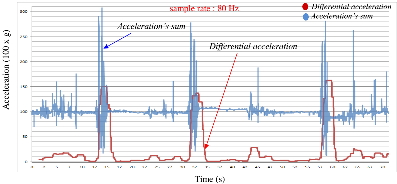
Figure 4. Fall signal.
