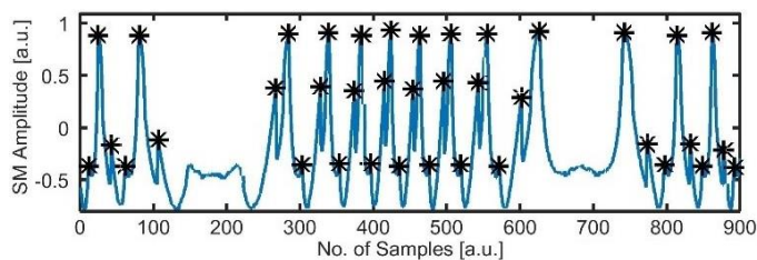
Fig. 11. True detected fringes (black stars) of exemplar multi-modal SM signal after the removal of all false detections, achieved at the end of Multi-Modal Processing Block.
