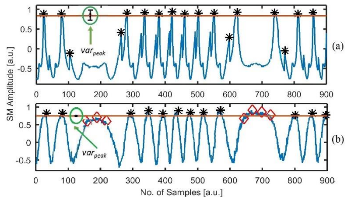
Fig. 8. (a-b) Detected peaks of exemplar SM signals with restrictive values of d_r = 5d and h_r . Horizontal red line represents mean value of amplitude of SM signal at detected peak locations while black vertical line encircled in green is representing var_{peak} value.
