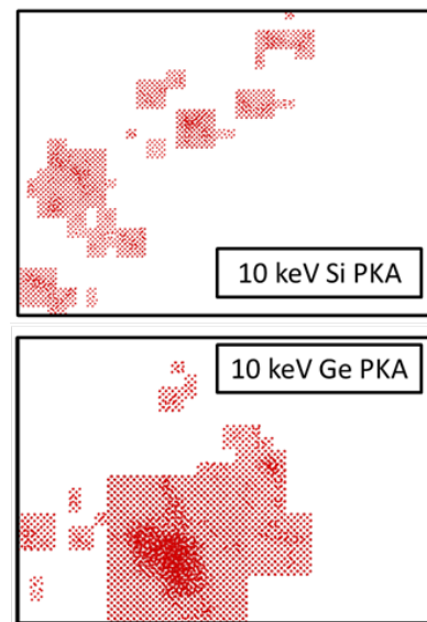
Fig. 14. Final defects observed in \text{Si}_{0.8}\text{Ge}_{0.2} after 10 keV Si PKA simulations (above) and 10 keV Ge PKA (below). Ge and Si atoms have the same color to make the defects and clusters easier to compare. There are around 400 defects in the Si PKA cascade and 1200 in the Ge cascade.
