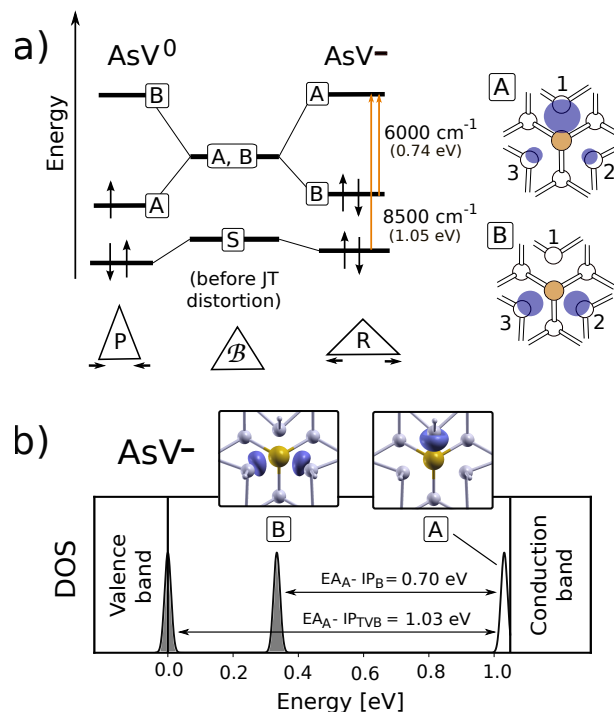
FIG. 2. Watkins' single-electron molecular orbital model 8,10 (no crystal field effects included), before and after Jahn-Teller (JT) distortions, measured optical bands 9 and their corresponding electronic-transition assignments within Watkins' model for \text{AsV}^- (a). Computed GW density of states for \text{AsV}^- at negative charge state is plotted in (b). Calculated optical absorption bands ( EA_A - IP_B and EA_A - IP_{TVB} ) for the \text{AsV}^- center 9 and their assignment to single-particle electronic transitions. In addition, the electronic density of the DFT-corresponding A and B states is also shown. DFT-corresponding Watkins' S state is strongly hybridized with the valence states.
