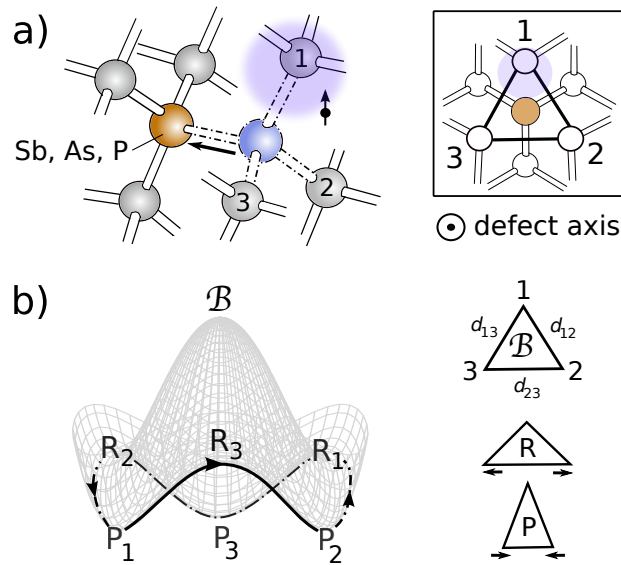
FIG. 1. The silicon E center: its projection along the vacancy-dopant axis (a) and Watkins et al. model for its potential energy surface at the neutral charge state (b). Three geometries for the E center are distinguished depending on the relative interatomic distances between atoms 1, 2 and 3: the symmetric breathing configuration ( \mathcal{B} ), the pairing configuration (P), and the resonant-bond configuration (R). P_i and R_i denote the pairing and resonant geometries with unpaired distances d_{jk} < d_{ij} = d_{ik} and d_{jk} > d_{ij} = d_{ik} , respectively.
