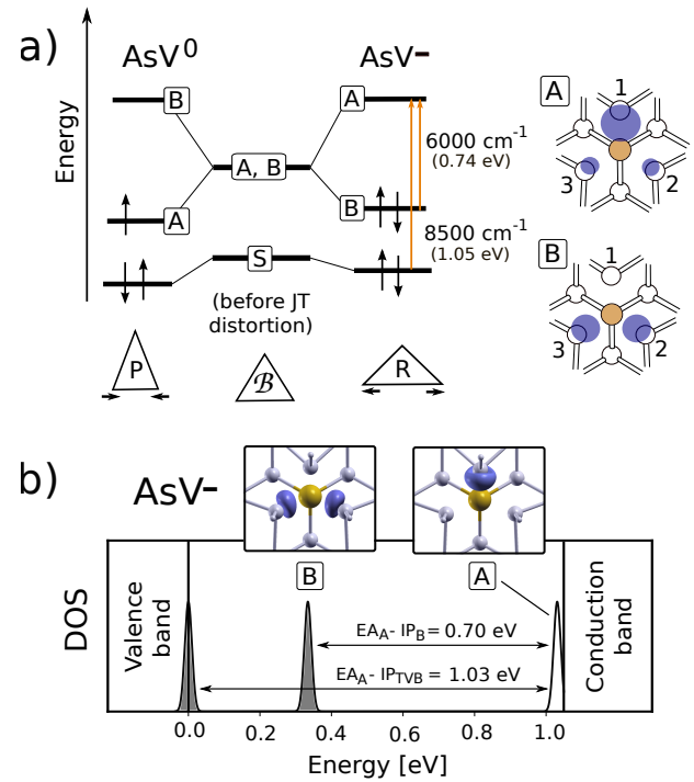
FIG. 2. Watkins' single-electron molecular orbital model 8,10 (no crystal field effects included), before and after Jahn-Teller (JT) distortions, measured optical bands 9 and their corresponding electronic-transition assignments within Watkins' model for \text{AsV}^- (a). Computed GW density of states for \text{AsV}^- at negative charge state is plotted in (b). Calculated optical absorption bands ( EA_A - IP_B and EA_A - IP_{TVB} ) for the \text{AsV}^- center 9 and their assignment to single-particle electronic transitions. In addition, the electronic density of the DFT-corresponding A and B states is also shown. DFT-corresponding Watkins' S state is strongly hybridized with the valence states.
