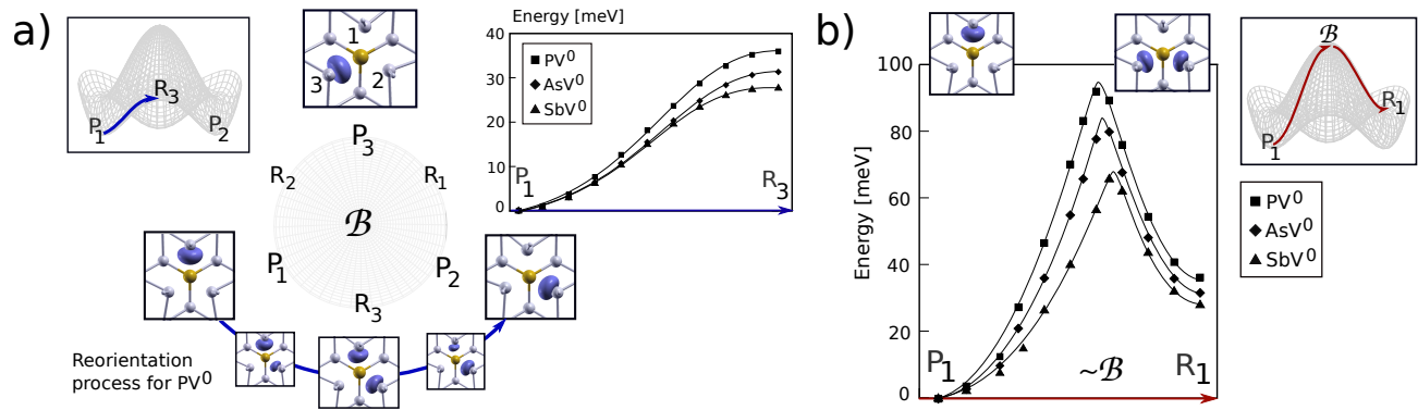
FIG. 3. Transition mechanism between pairing configurations, P, (a) and potential energy surface (b) of E centers at neutral charge state. The electronic density for the unpaired electron at different atomic configurations is also shown. Points are obtained within the CI-NEB algorithm (a) and single point DFT calculations (b). Lines are a guide for the eye.
