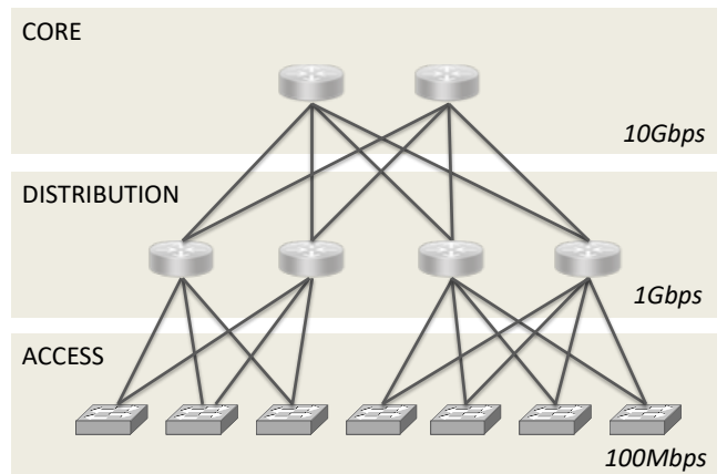
Figure 13 - campus network
