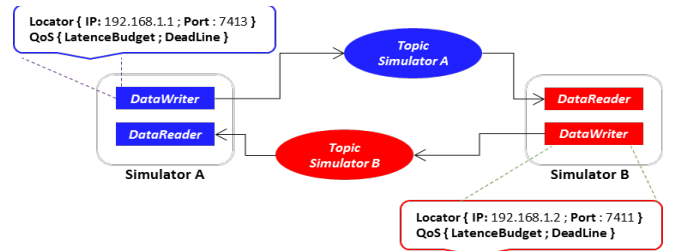
Figure 7 – DDS view of the considered application
