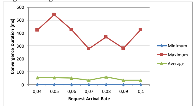
Figure 16 – Convergence duration
