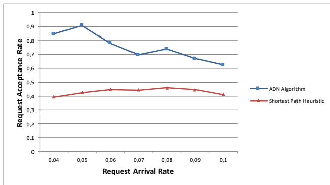
Figure 17 – Requests Acceptance Rate
