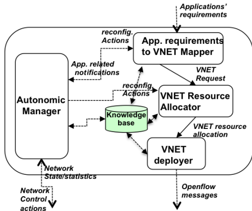
Figure 5 - ADN's functional components
