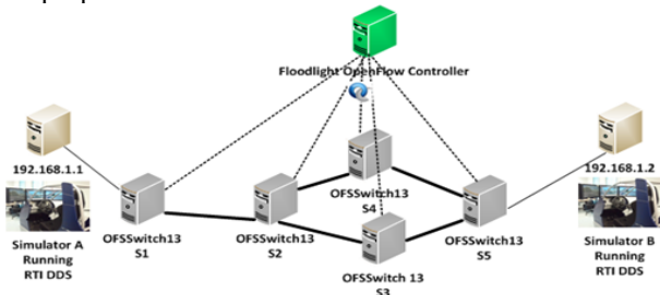
Figure 6 - Testbed environment
