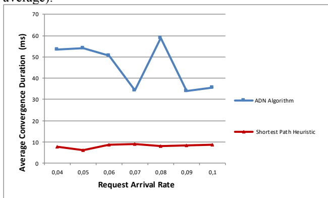
Figure 18 – Convergence duration
