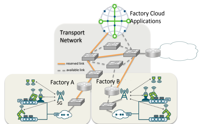
Figure 1 - Industry 4.0 networks
