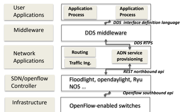
Figure 4 - "ADN service provisioning" network function
