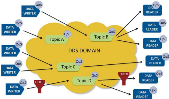
Figure 2 - Data Distribution Service overview
