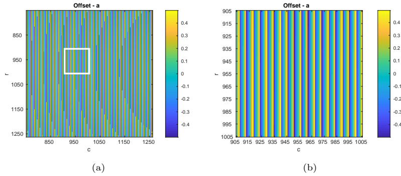
Figure 14: a) Offset a for each camera pixel, determined by the calibration functions, b) close up on region marked by white box.
