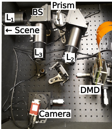
Figure 3: System prototype
