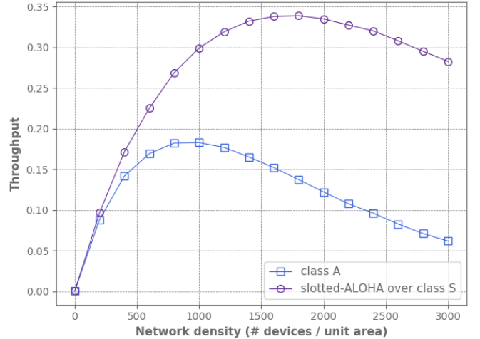
Fig. 2: Network throughput of Class A and Class S LoRaWAN deployments.
