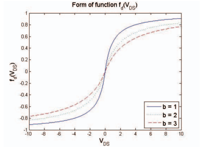
Fig. 2. Curves of the function f_d(V_{DS}) with different values of b .
