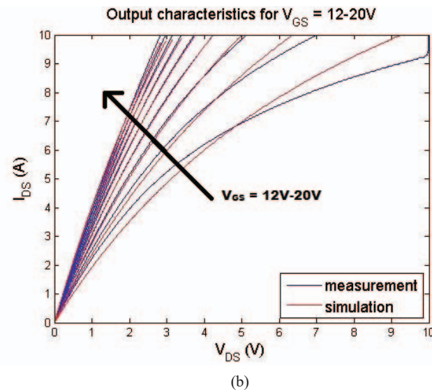
Fig. 3. SiC MOSFET forward output characteristics: simulation vs measurement (a) SCT50N120, (b) SCT2280KE.
