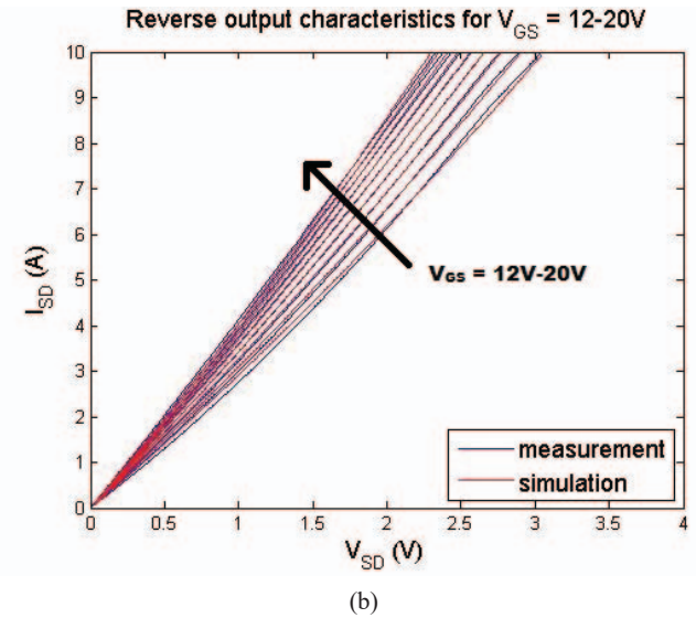
Fig. 4. SiC MOSFET reverse output characteristics: simulation vs measurement (a) SCT50N120, (b) SCT2280KE.
