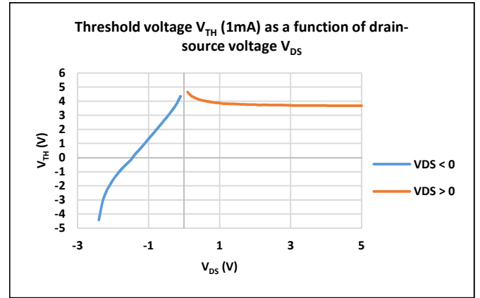
Fig. 7. Threshold voltage V_{TH} as a function of the drain-source voltage V_{DS} (here, the threshold voltage is defined as the minimum value of the gate bias voltage that allows a current of 1mA across the MOSFET at a fixed drain-source voltage).
