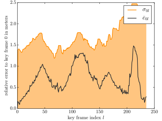
(b) Relative errors with respect to keyframe 0 (● above). Ground truth \bar{e}_{0l} is drawn in black, the shaded orange area covers the predicted 1- \sigma standard deviation \sigma_{0l} .
