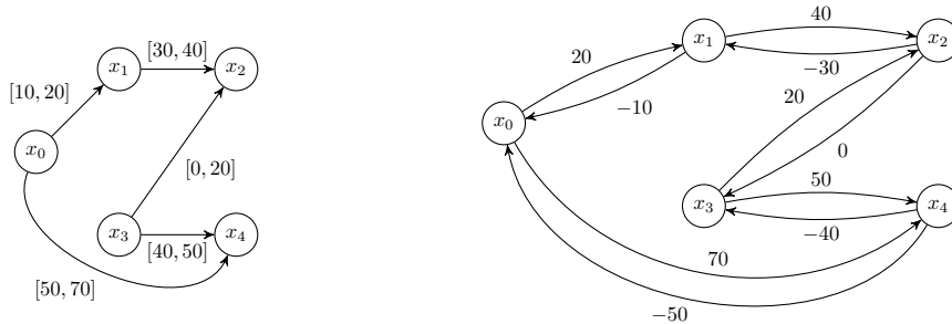
Figure 1: Simple Temporal Problem: constraint graph (on the left) and distance graph (on the right).
