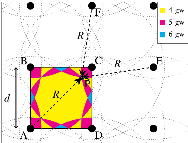
Fig. 13. Square deployment with \frac{3\sqrt{2}}{5} , L = 1, 2, 3, 4 .
