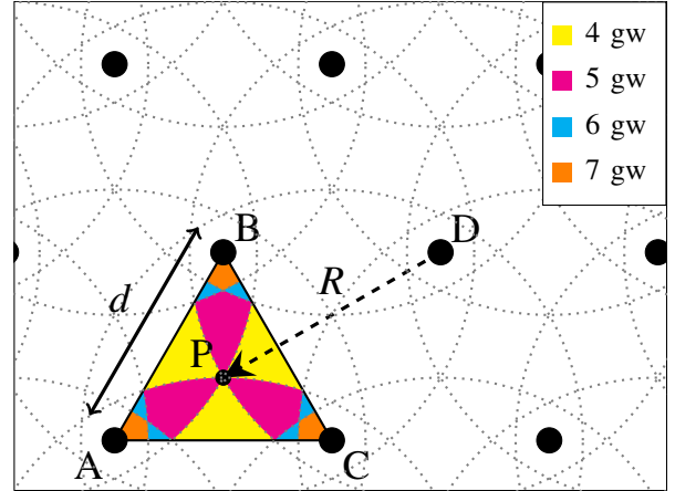
Fig. 9. Honeycomb deployment with d = \frac{\sqrt{3}}{2}R , L = 1, 2, 3, 4 .
