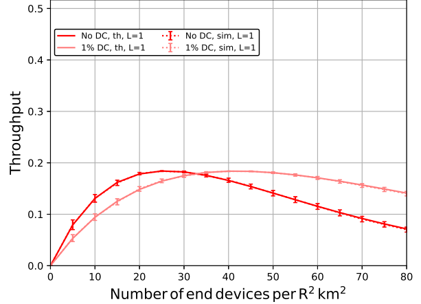
Fig. 4. Throughput in single-gateway deployments.
