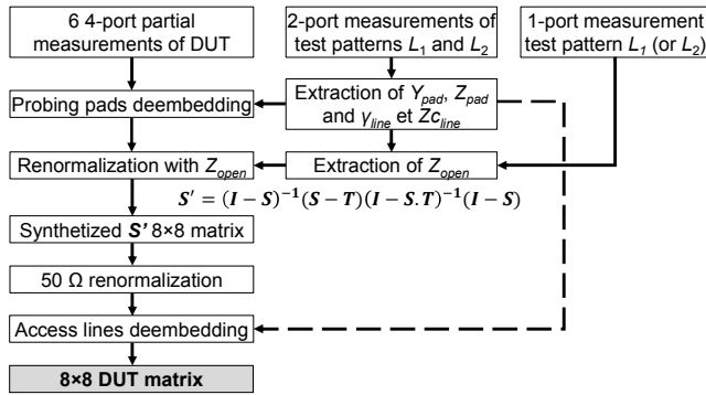
Fig. 1. Illustration of the deembedding procedure.
