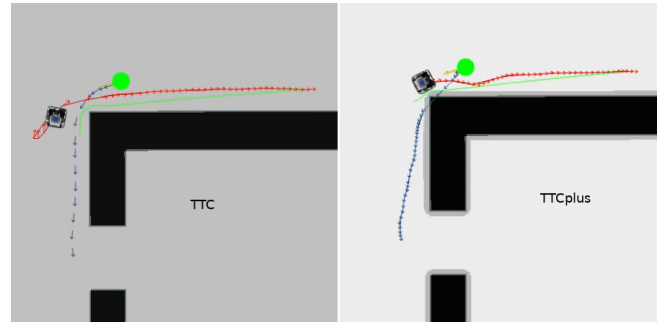
Fig. 7. The original TTC constraint-based trajectory shown on the left results in unnecessary oscillations due to exaggerated constraint. However, TTCplus constraint regulates this exaggeration and results in a smooth trajectory as shown on the right. Note that the trajectory on the left is making the robot move backwards even when there is no necessity. Red: Robot Trajectory, Blue: Human Trajectory.
