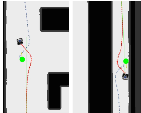
Fig. 2. Robot getting stuck due to entanglement of trajectories. The blue trajectories correspond to human trajectories, and the red ones correspond to robot trajectories. In both situations shown, there exists an alternate solution for the robot to solve the problem. However, the assumption that human is always moving and the constraint of proxemics makes the robot wait in the same entanglement, speculating the motion of human. The picture on left is of open space, whereas the one on the right is of a narrow corridor.
