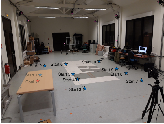
Fig. 7. Experimental setup to capture human trajectories
