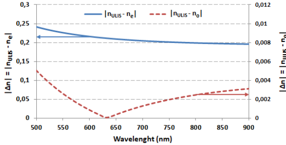
Fig.11. Difference between the ULIS resin refractive index and liquid crystal E7 considering extraordinary index (blue plain line, left Y axis) and ordinary index (red dashed line, right Y axis). Refractive index of ULIS resin was measured by ellipsometry while E7 liquid crystal dispersion curves are derived from extended experimental measurements by a three-coefficient Cauchy model (Li and al. 2005).
