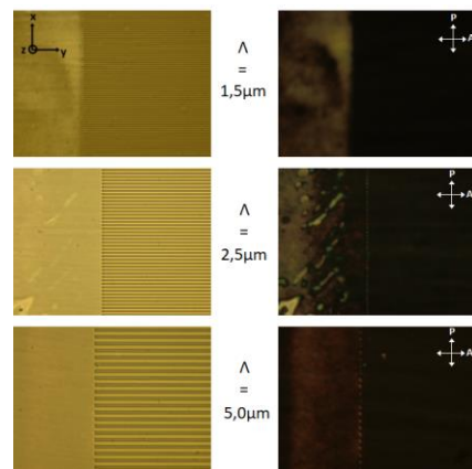
Fig. 5. Optical microscopy observation (x50) of LC-impregnated diffraction gratings with period from 1.5 to 5.0µm and 840nm depth without polarizers (in left) and between cross polarizers (in right). As expected for aligned LCs, transmission is extinguished between crossed polarizers.
