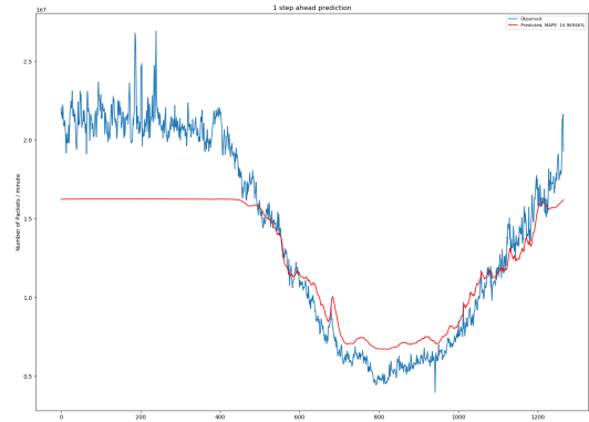
(b) Prediction Result of LSTM model
