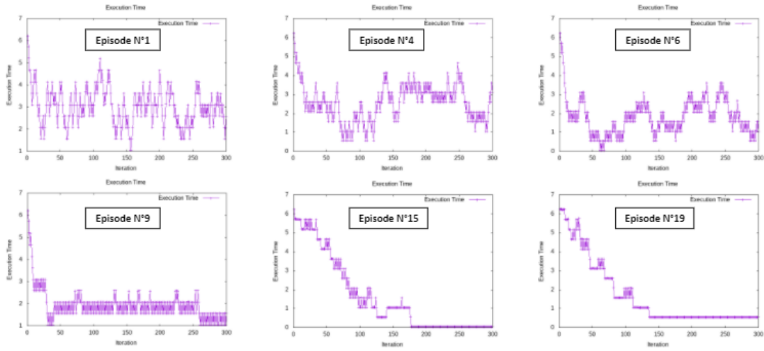
Figure 5.3: Convergence Performance using a second Reward Function
