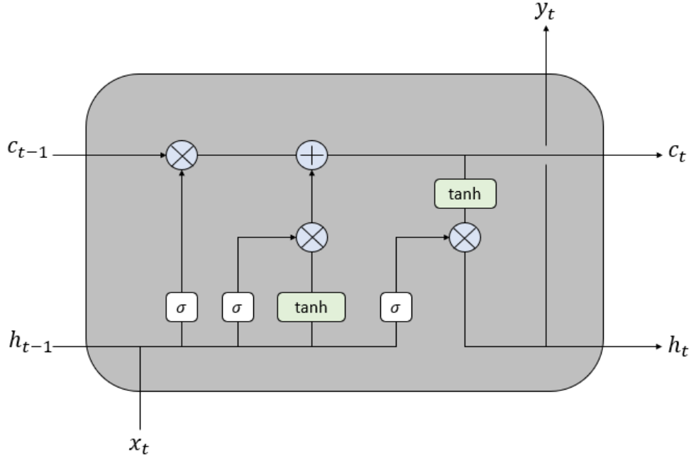
Figure 3.3: LSTM Cell
