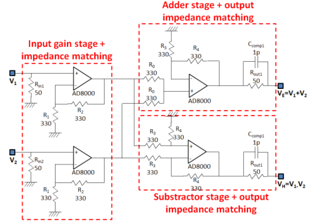
Fig. 2. Schematic of the proposed electronic coupler
