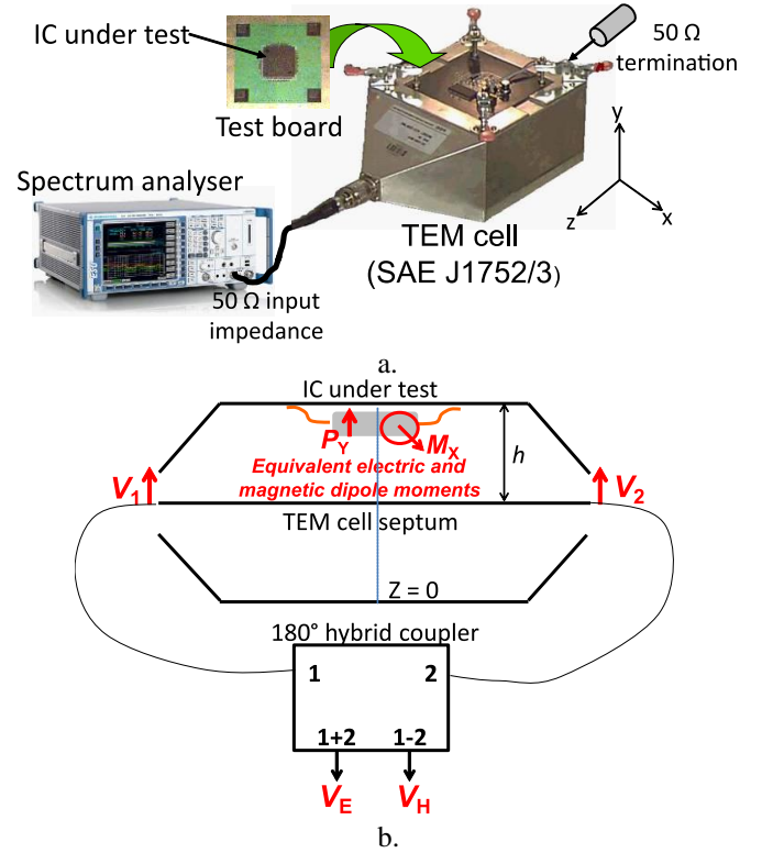
Fig. 1. a. Typical IC radiated emission measurement set-up; b. Extraction of the electric and magnetic-field coupling induced voltages
