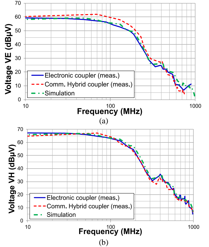
Fig. 5. Line under test terminated by 50 \Omega . Comparison between measurements with the proposed electronic coupler, a commercial 180° hybrid coupler and simulation of: (a) E-field coupling induced voltage V_E , (b) H-field coupling induced voltage V_H
