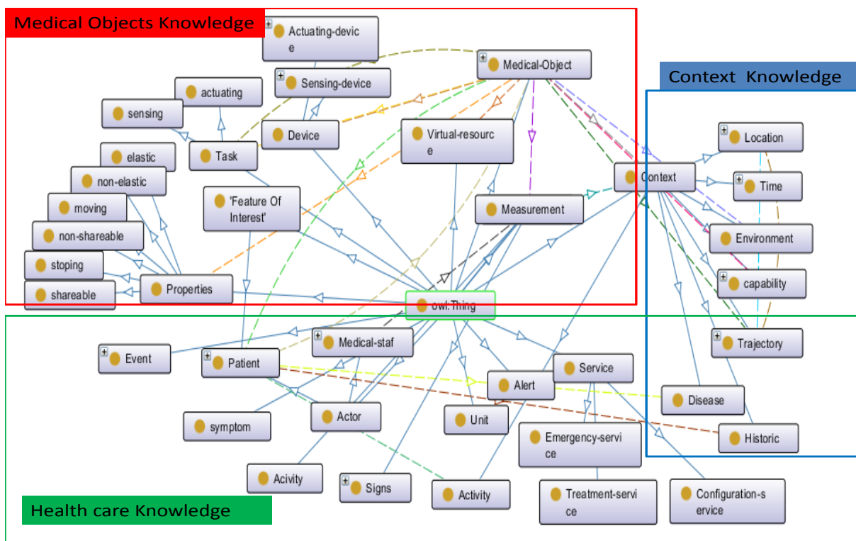
FIGURE 3 HealthIoT Ontology
