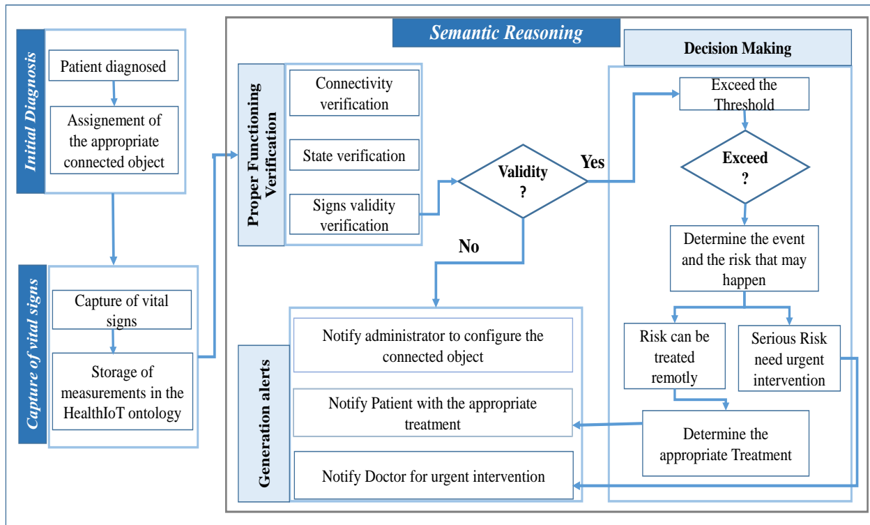
FIGURE 4 Reasoning Process.
