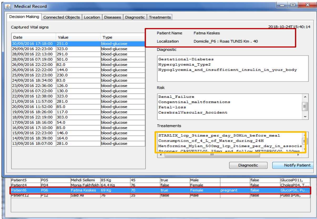
FIGURE 8 Decision Making
