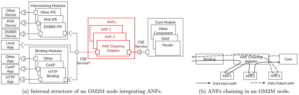
Figure 10: Seamless integration in the OM2M IoT platform.
