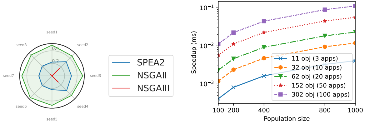
(a) Hyper-volume measure on the formulated problem with C_p = 100\% ; M_p = 100\% ; N = 200 , l = 28 . (b) Speedup achieved by the NSGAII-based evolutionary strategy on the formulated problem for 3, 10, 20, 50 and 100 IoT applications (on a Processor Intel (R) Core (TM) i7-7500U CPU @2.70GHz).
