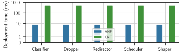
Figure 3: Traffic Control Functions deployment time.
