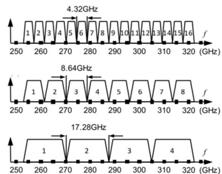
Fig. 2. Possible band allocation above 275 GHz.
