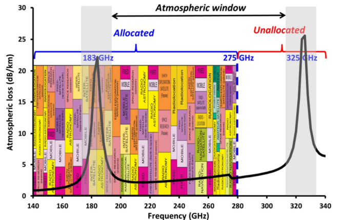
Fig. 1. Atmospheric loss [1] and band allocation [2]-[3] for millimetre-wave applications in G-band.
