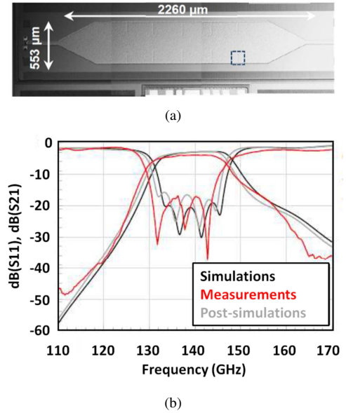
Fig.5. 140 GHz 4 th -order SIW filter with 10% relative-bandwidth: (a) photography and (b) simulated (HFSS) and measured results.
