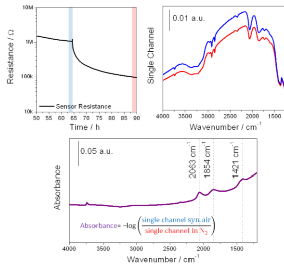
Figure 2. Resistance measurement and simultaneously attained single channels spectra of a \text{WO}_3 film during exposure to dry synthetic air (blue) and nitrogen (red) at 300 °C. By referencing the single channel spectrum in dry synthetic air to the one in nitrogen, the absorbance spectrum was attained.
