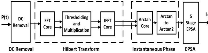
Fig. 13. Block diagram of FPGA based hardware emulation of IEPs.
