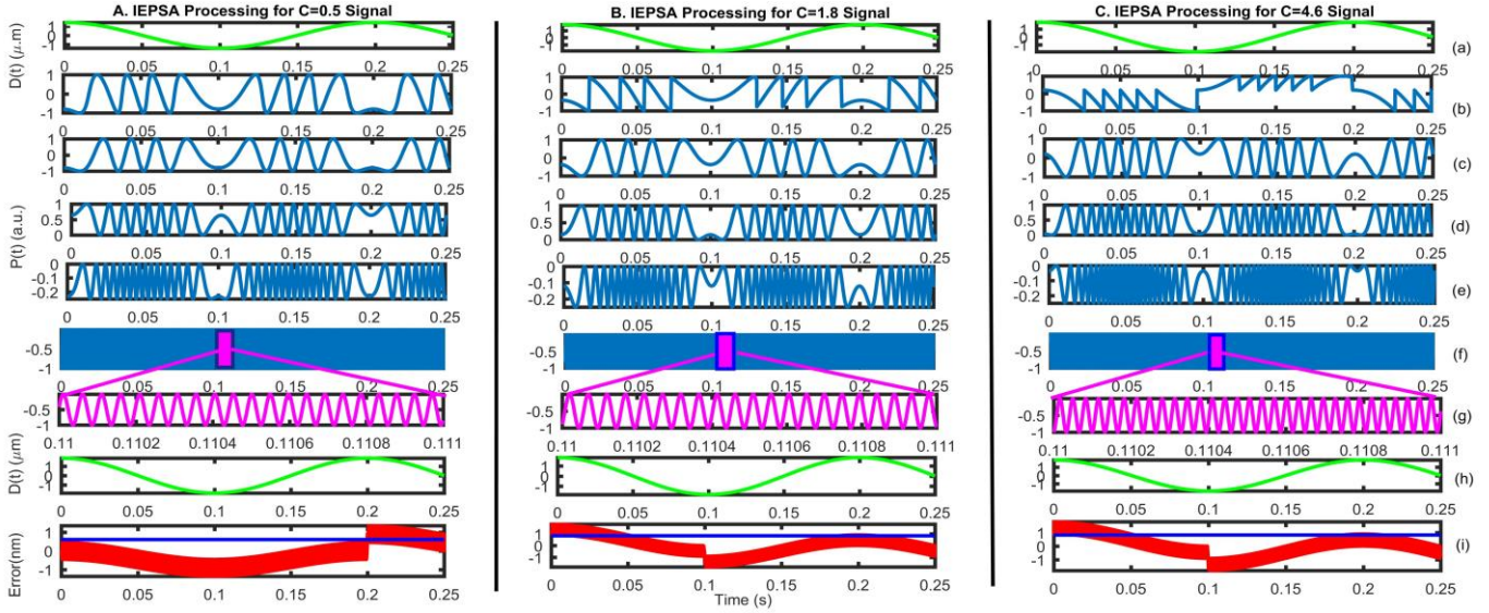
Fig. 12. IEPSA response for simulated SM signals for (A) weak feedback regime ( C=0.5 ), (B) moderate feedback regime ( C=1.8 ) and (C) strong feedback regime ( C=4.6 ). (a) target displacement D(t) (b) P(t) , (c) fringe reshaping, (d) P_2 , (e) I_0 , (f) I_0 , (g) zoomed view of I_0 , (h) retrieved target displacement by fringe counting and (i) peak-peak error (red line) and RMS error (blue line) between reference displacement and retrieved displacement.
