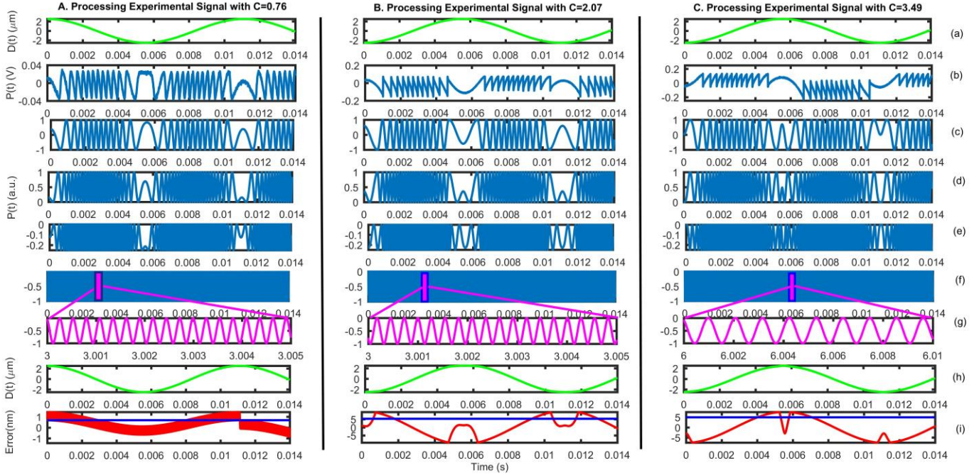
Fig. 14 IEPSA results for experimental SMI signals for (A) C=0.76 , (B) C=2.07 and (C) C=3.49 , (a) acquired target displacement D(t) from reference PZT sensor (b) P_1(t) , (c) fringe reshaping, (d) P_2 , (e) I_0 , (f) I_1 , (g) zoomed view of I_2 , (h) retrieved Displacement by fringe counting and (i) peak-peak error (red line) and RMS error (blue line) between PZT displacement and retrieved displacement
