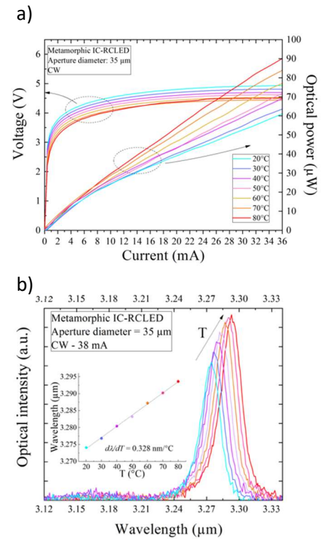
Figure 7 a.) CW P – I – V characteristic and b) electroluminescence spectra for an IC-RCLED with a 35 μm diameter aperture given at different temperatures. Inset shows the temperature dependence of the wavelength. Solid line represents a linear fit to the data.
