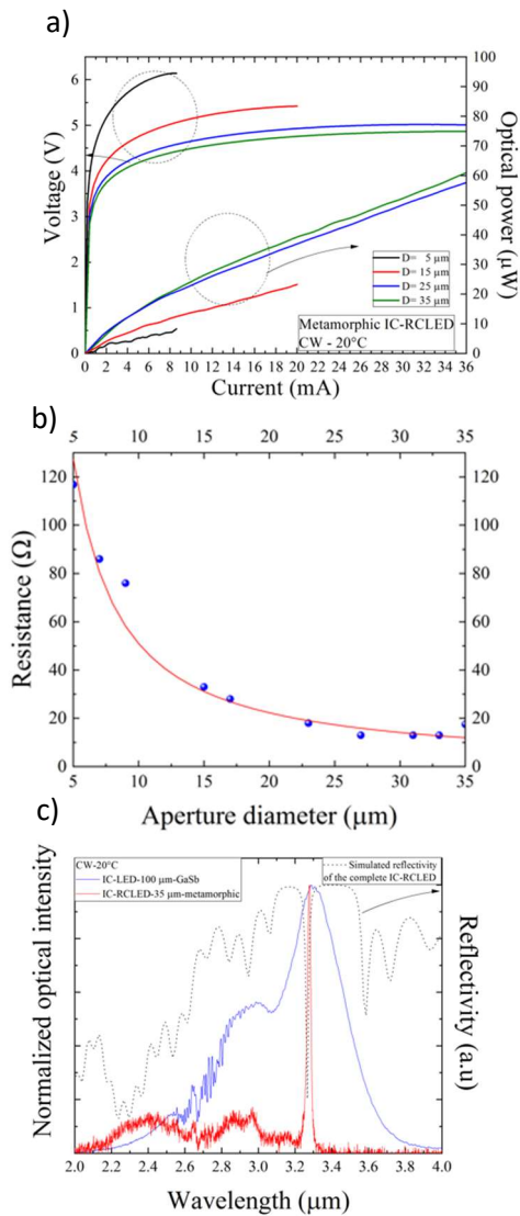
Figure 6. (a) CW L – I – V characteristics, and (b) series resistance for RCLEDs as a function of the aperture diameter ranging from 5 μm to 35 μm. (c) Emission spectra of a 35 μm oxide aperture IC-RCLED and 100 μm mesa diameter IC-LED at 20°C in CW and simulated reflectivity of the whole IC-RCLED
