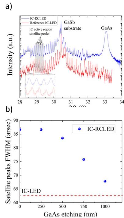
Figure 2. a) \omega -2 \theta HRXRD scans at the (0 0 4) reflection for the RCLED and reference LED structure. Inset: magnification on the satellite peaks – b) Evolution of the FWHM of the satellite peaks of the RCLED with etched GaAs.
