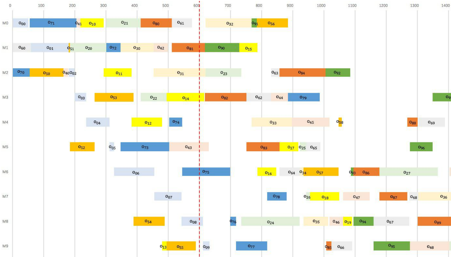
Fig. 13. The Gantt chart of the best-found solution of the original schedule for the M10 based EDJSP
