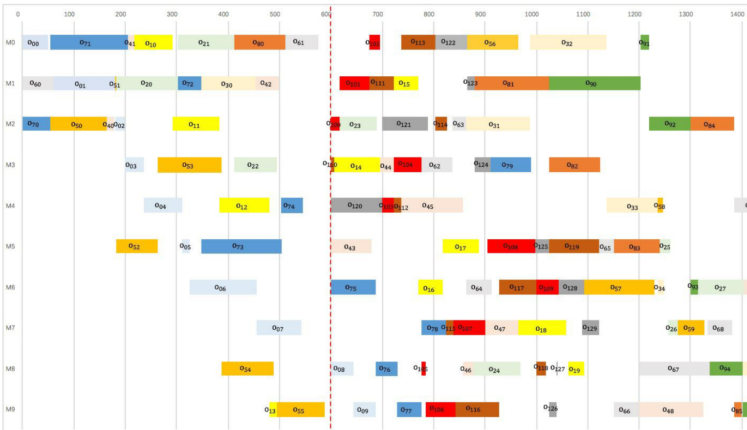
Fig. 14. The Gantt chart of the best-found solution of the updated schedule for the M10 based EDJSP
