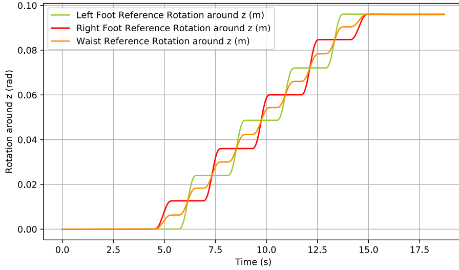
Figure 14: Waist rotation parameter during simulation is now correctly updated as the average between the feet orientation – Output of the PG entity
