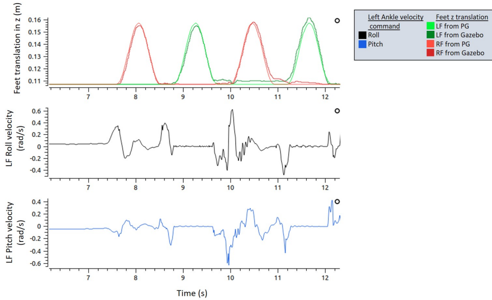
Figure 18: Ankle controller velocity output. Pyrène walks on the stick at time 9.6s – The ankle controller gain is set at 0.01 – The controller is not yet plugged to the SoT.
