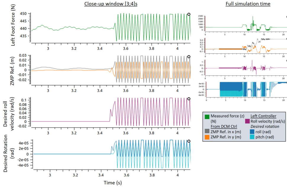
Figure 21: Oscillatory behaviour – Full simulation and close-up with an ankle admittance control gain of 0.01 rad.m/N. The oscillations start at time 3.45s when the controller gain is switched from 0 to 0.01 after initialization. Most variables of the control scheme oscillate with the controller.
