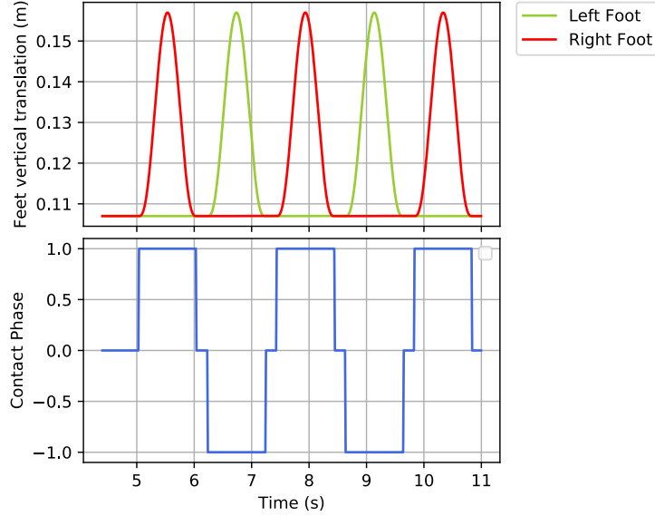
Figure 19: Output Contact Phase Signal from the PG – 0 stands for DSP, 1 for LF support and -1 for RF support
