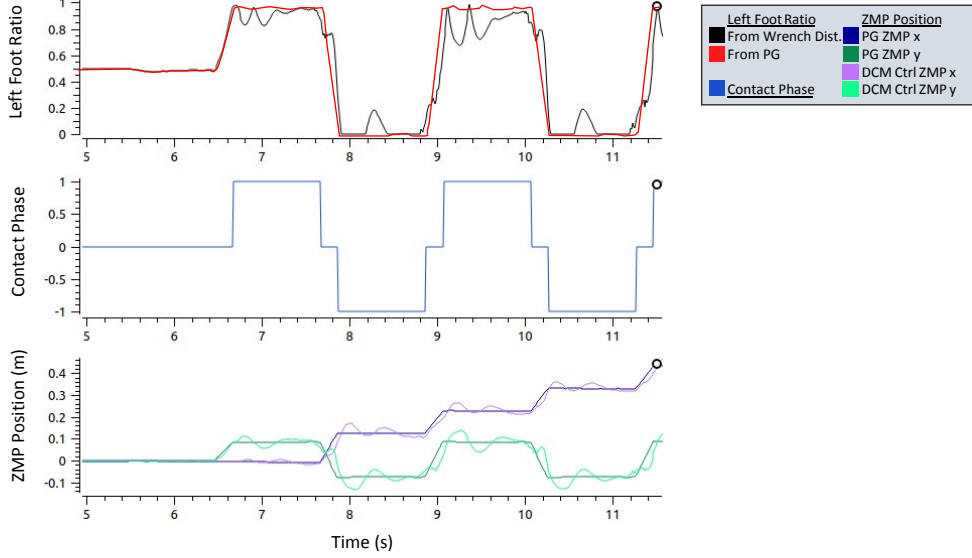
Figure 20: Top: Left foot ratio signal as now implemented in the Wrench Distribution entity (in black); the red curve shows what an ideal ratio would look like, it takes the ZMP trajectory of the WPG directly instead of the one adapted by the DCM controller. Middle: Contact Phase Signal. Bottom: ZMP trajectories that explain the Left foot ratio shape: the DCM controller actually computes a rather important correction.
