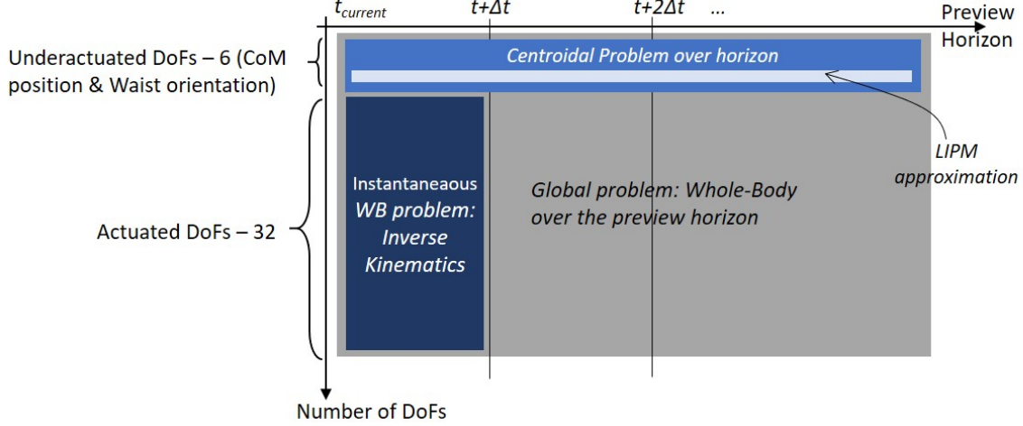
Figure 5: Scheme of the complexity of the locomotion problem for humanoid robots, based on [Naveau, 2016]. Being able to solve the full problem in the grey rectangle (whole-body trajectory for the full preview future) is a long-run objective. For now though, this problem is impossible to solve in milliseconds. At this speed, it is however possible to solve the dark blue problem: whole-body problem but only for the nearest future, as well as the linearized problem at the level of the Center of Mass only, over the full 1.6 s preview.
