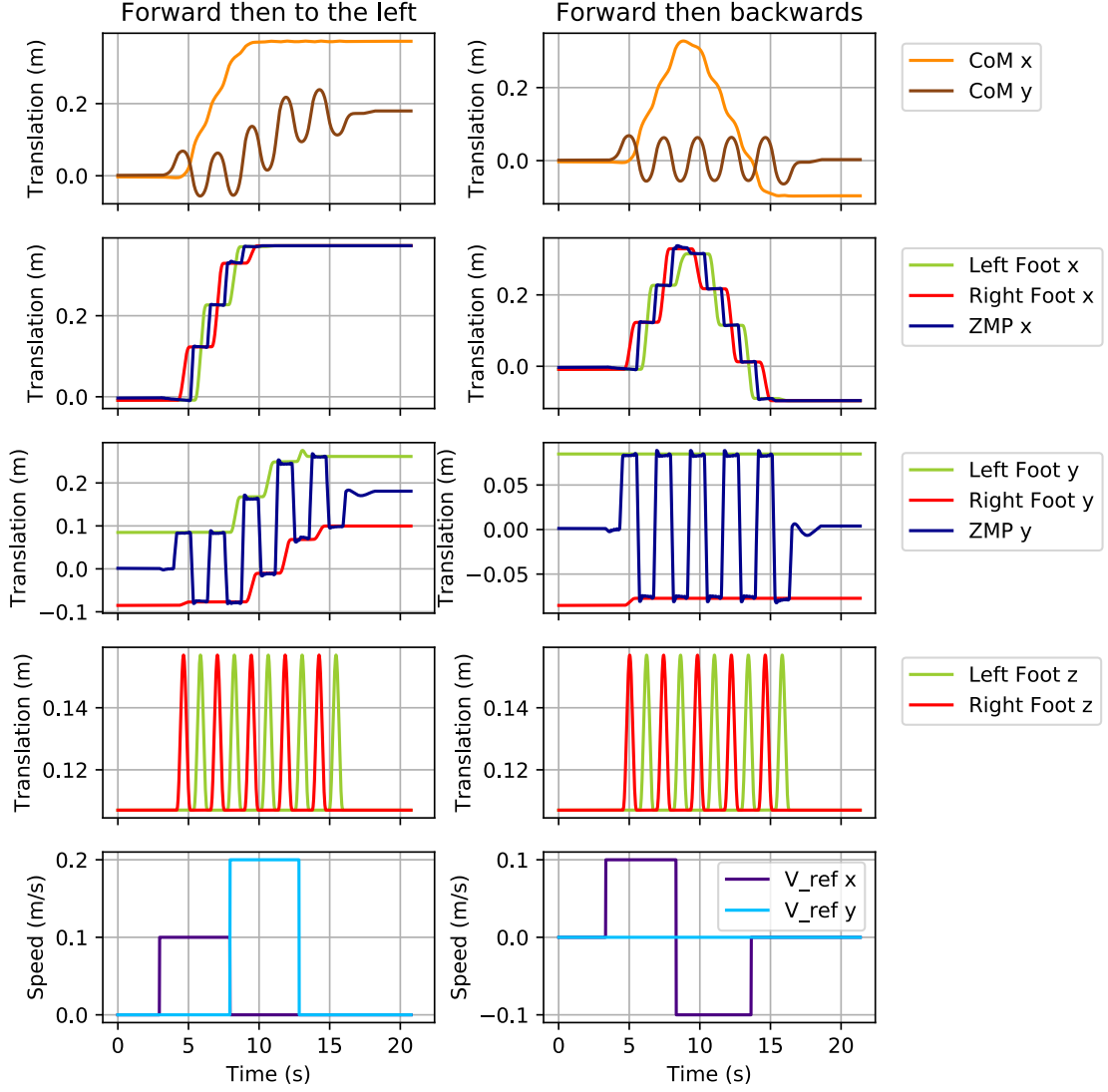
Figure 12: Reference trajectory computed by the PG in the online simulation, cases of direction transitions, stop at the end of the motion. Left: Forward motion - V_{ref} = (0.1, 0.0, 0.0) - then to the left - V_{ref} = (0.0, 0.2, 0.0) . Right: Forward motion - V_{ref} = (0.1, 0.0, 0.0) - then backwards - V_{ref} = (-0.1, 0.0, 0.0)
