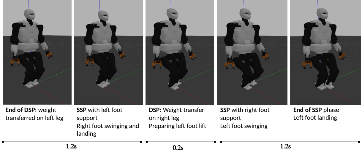
Figure 11: Time lapse images of the robot executing two steps forward at 0.1 m/s speed ( V_{des} = (0.1, 0.0, 0.0) ). DSP stands for Double Support Phase and SSP stands for Single Support Phase.
