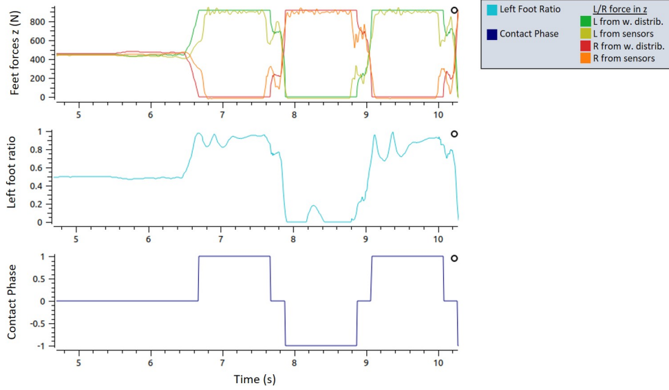
Figure 22: Top: Surface vertical force computed by the wrench distribution and measured by the force sensors (the measured wrench is filtered by the feet sensors calibration at this point). The force increase measured during the DSP is mainly due to a rather strong impact force. Middle: Left foot ratio. Bottom: Contact phase.
