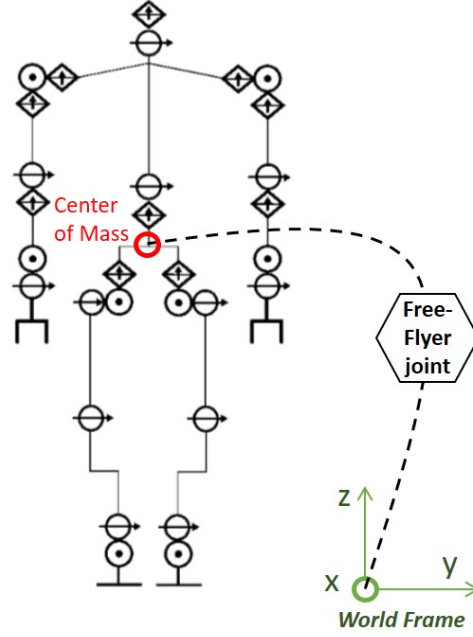
Figure 4: Joint distribution on Pyrène – each of the robot’s joints allows one Degree of Freedom, to which a special free-flyer joint is added, that links the robot to the world frame
