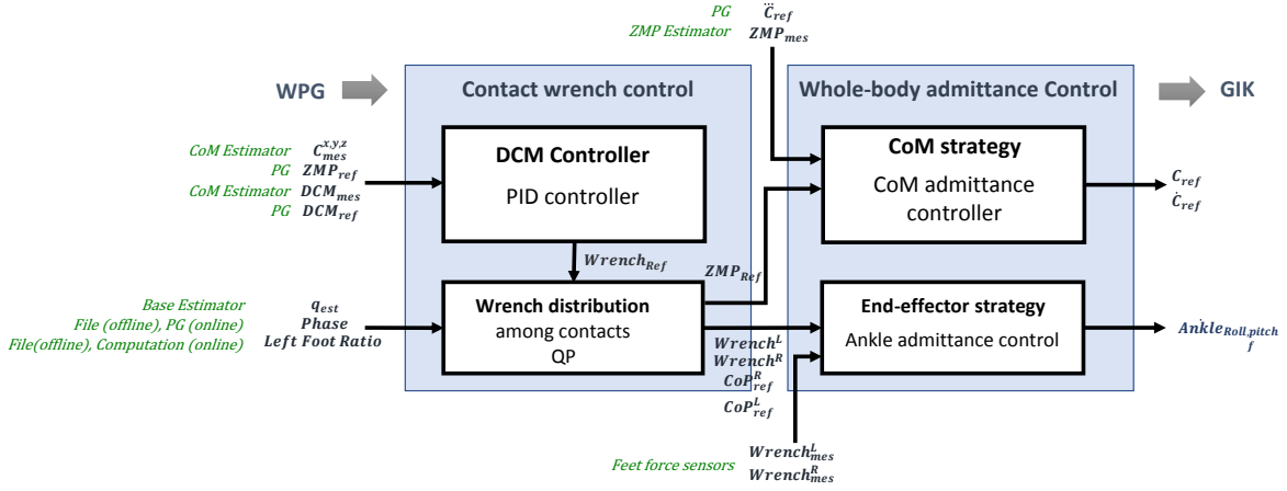
Figure 16: Full Stabilizer scheme – the green scriptions indicate which entities the facing signals come from. The Wrench distribution and End-effector strategy (Ankle admittance control) entities are the two entities added to the stabilizer during the internship.
