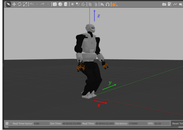
Figure 9: View of Talos in Gazebo in a world with only a floor and gravity force – Talos is in half-sitting position, corresponding to its initial state and at the origin of the simulation world. The three directions of motions are respectively x – to the front, y – to its left, and z – to the top.
