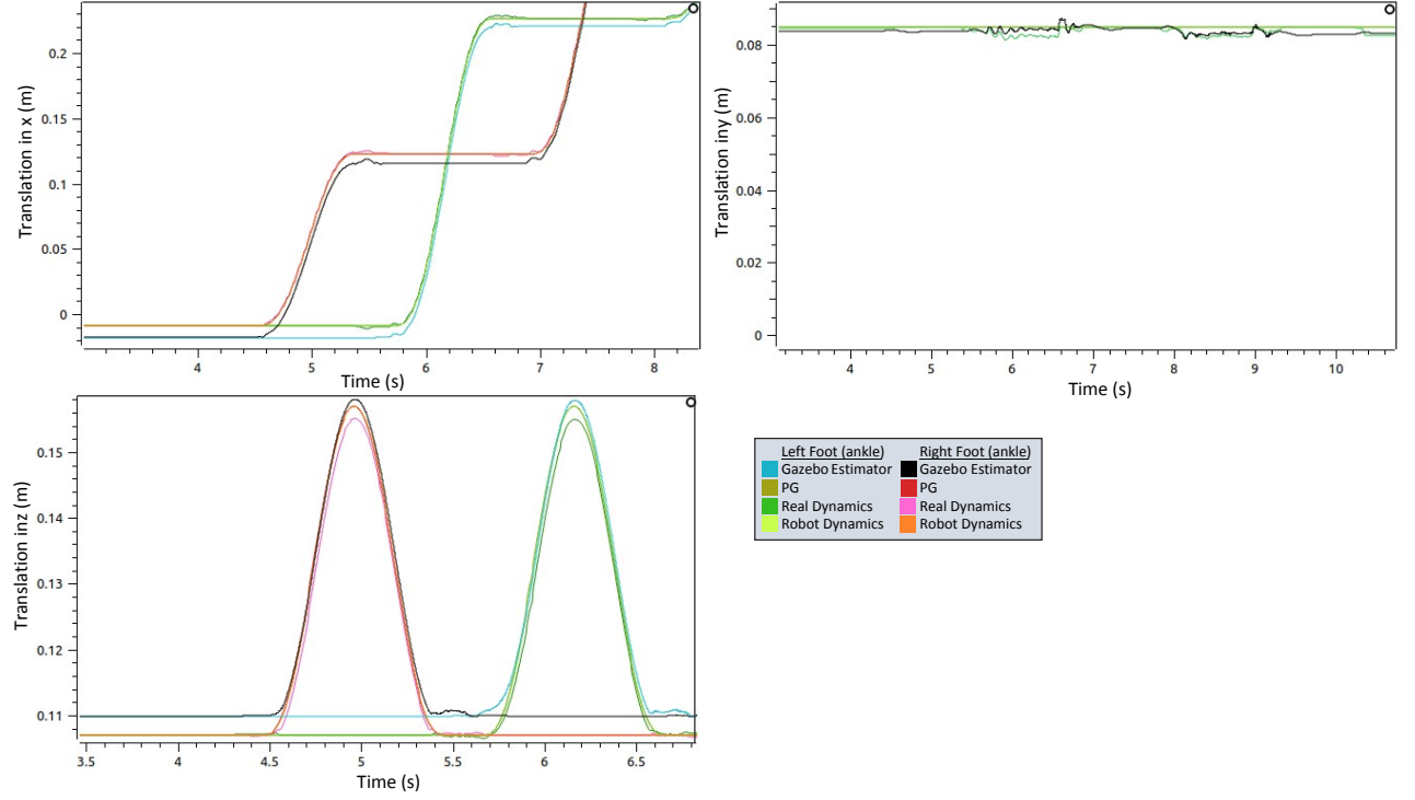
Figure 15: Feet translation values for the feet in the initial state (until 4.5s) then during the walk between the different estimators and the PG. There is almost no difference between the PG and the estimators of the control scheme, but a larger one with Gazebo's estimator.
