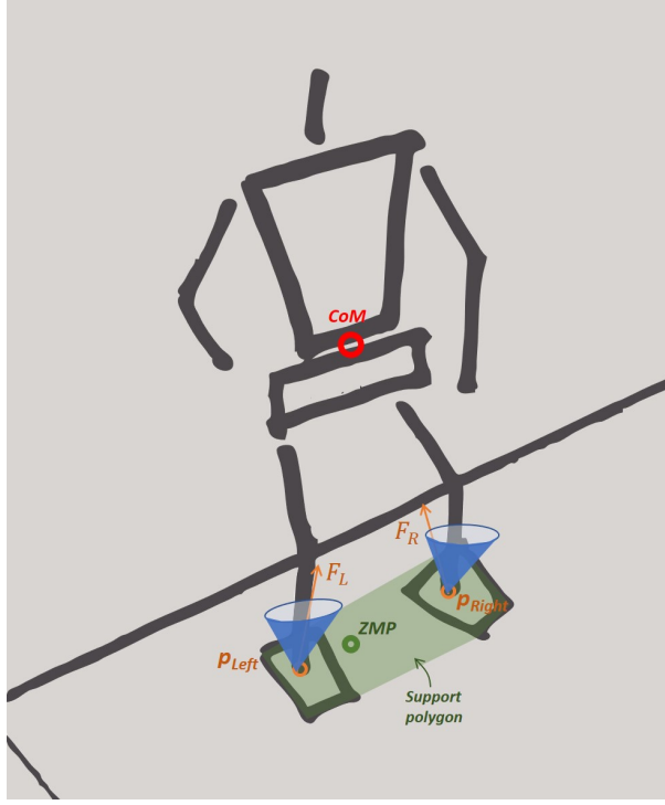
Figure 6: Scheme of the contact forces expressed at points p_i of each foot and the associated contact wrench cones ; the convex polygon of contact and the ZMP lying in it
