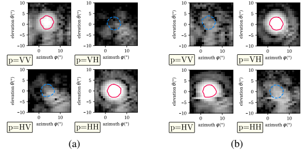
Fig. 6. Isolines generated in the azimuth/elevation planes at the range R=9.3\text{m} at the location of the sensor 2 ( scenario 2 ) when the two-port sensor is replaced by: (a) an open-circuit at each input port of the two sensor antennas, and (b) by an impedance-matched transmission line. Dark to bright colors in the figures indicate low (-90dB) to high (-60dB) radar echo levels.
