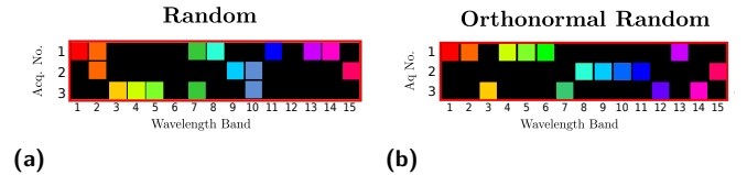
Fig. 3. Example of spectral filter where N = 3 , and W = 15 . DMD mask type is a) random b) random orthonormal.
