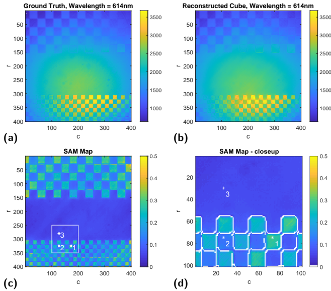
Fig. 16. a) Monochromatic image at 614nm for the ground truth, b) corresponding monochromatic image for the reconstructed cube, c) map of the SAM for the reconstructed data for scene B, d) close up the SAM map with edges overlaid.
