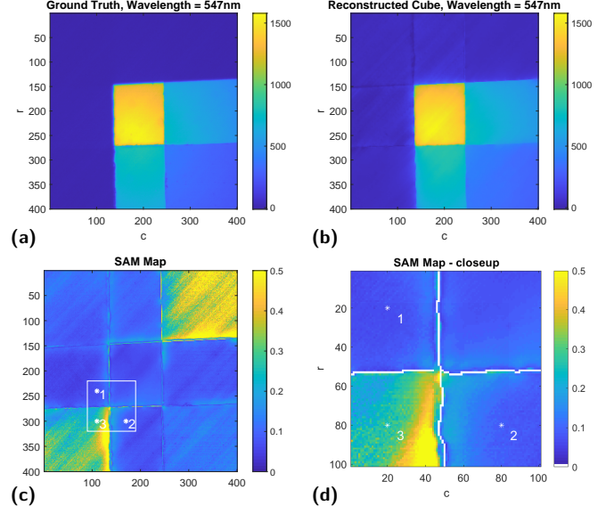
Fig. 13. a) Monochromatic image at 547 nm for the ground truth, b) corresponding monochromatic image for the reconstructed cube, c) map of the SAM for the reconstructed data for scene A, d) close up of scene A SAM map with edges overlaid.
