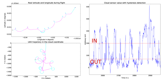
Fig. 8. Top left corner : real lat long plot of a flight section ; Bottom left corner: trajectory of the UAV in the cloud origin in meters (cyan/purple = outside/ inside); Right: Cloud sensor value getting during this section
