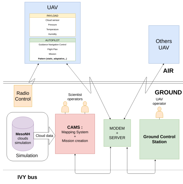
Fig. 2. The global system architecture
