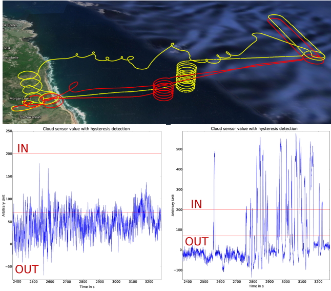
Fig. 6. Trajectories from a flight with 2 UAVs and the cloud sensor values (red trajectory corresponds to left plot and yellow trajectory to right plot). The horizontal lines are detection threshold with hysteresis, crossing upper line is entry detection, going back below bottom line is exit detection.
