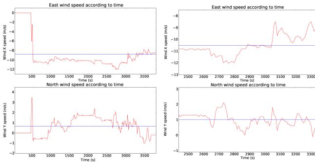
Fig. 7. Extracted relative wind during an entire flight at the left and a laps of time on the right
