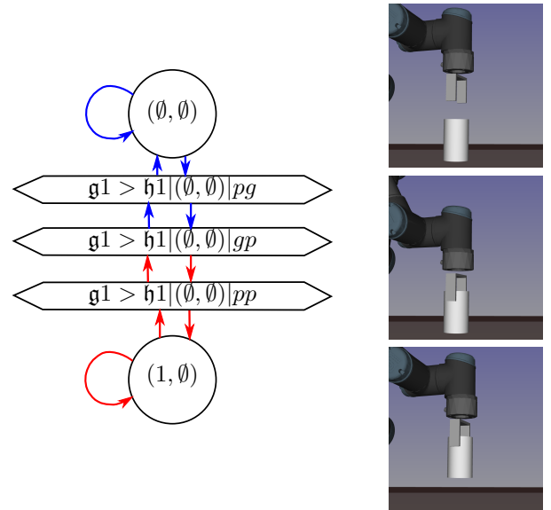
Figure 6. Along a transition where an object in placement is grasped by a gripper, we add three waypoint states called pregrasp ( pg ) where the gripper is above the object, grasp-placement ( gp ) where the object is grasped but still in placement and preplacement ( pp ) where the object is grasped above the contact surface. All transitions between the state with the least active grasps and the waypoint gp have the same constraints as the loop transition of the state with the least active grasps (here: place_{e1} and place_{e1}/comp in blue). All transitions between the waypoint state gp and the state with the most active grasps have the same constraints as the loop transition of the state with the most active grasps (here: grasp_{11} and grasp_{11}/comp in red).
