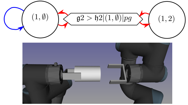
Figure 5. Along a transition where an object already grasped is grasped by an additional gripper, an intermediate waypoint state called pregrasp ( pg ) is added. This intermediate state is represented by a hexagonal box. g2 > h2|(1, \emptyset)|pg means that gripper 2 is going to grasp handle 2 from the state where gripper 1 grasps handle 1. The constraints associated to this waypoint state are the constraints of the state with the least active grasps (here (1, \emptyset) ) and the pregrasp constraint corresponding to the grasp that is added in the node with the most active grasps (here pregrasp_{22} ). The transition constraints are the same for all transitions (in red) and the same as the loop transition of the state with the least active grasps (in blue: here grasp_{11} and grasp_{11}/comp ).
