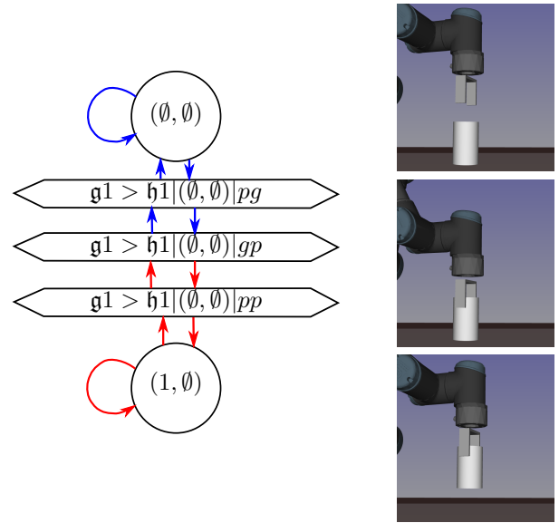
Figure 6. Along a transition where an object in placement is grasped by a gripper, we add three waypoint states called pregrasp (pg) where the gripper is above the object, grasp-placement (gp) where the object is grasped but still in placement and preplacement (pp) where the object is grasped above the contact surface. All transitions between the state with the least active grasps and the waypoint gp have the same constraints as the loop transition of the state with the least active grasps (here: place_1 and place_1/comp in blue). All transitions between the waypoint state gp and the state with the most active grasps have the same constraints as the loop transition of the state with the most active grasps (here: grasp_{11} and grasp_{11}/comp in red).
