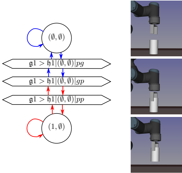
Fig. 6. Along a transition where an object in placement is grasped by a gripper, we add three waypoint states called pregrasp ( pg ) where the gripper is above the object, grasp-placement ( gp ) where the object is grasped but still in placement and preplacement ( pp ) where the object is grasped above the contact surface. All transitions between the state with the least active grasps and the waypoint gp have the same constraints as the loop transition of the state with the least active grasps (here: place 1 and place 1/comp in blue). All transitions between the waypoint state gp and the state with the most active grasps have the same constraints as the loop transition of the state with the most active grasps (here: grasp 11 and grasp 11/comp in red).
