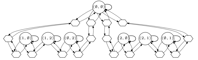
Fig. 7. Structure of the constraint graph corresponding to the system in Section V-D2 after inserting waypoint transitions. Waypoint transitions starting from/going to (\emptyset, \emptyset) contain three waypoint states. All other waypoint transitions contain one waypoint state.
