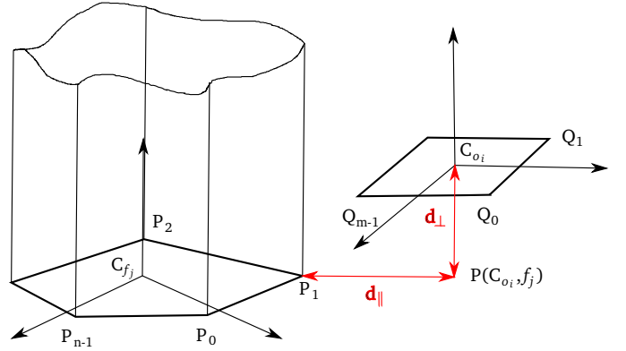
Fig. 2. Distance defined by two convex polygons.
