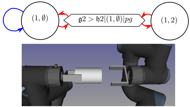
Fig. 5. Along a transition where an object already grasped is grasped a second time, an intermediate waypoint state called pregrasp (pg) is added. This intermediate state is represented by a hexagonal box. g2 > h2|(1, \emptyset)|pg means that gripper 2 is going to grasp handle 2 from the state where gripper 1 grasps handle 1. The constraints associated to this waypoint state are those of the state with the least active grasps (here (1, \emptyset) ) and the pregrasp constraint corresponding to the new grasp (here pregrasp 22 ). The transition constraints are the same for all transitions (in red) and identical to the loop transition of the state with the least active grasps (in blue: here grasp 11 and grasp 11/comp ).
