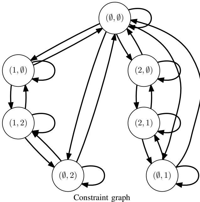
Fig. 1. Example of manipulation planning problem. Top: two UR3 robots with one gripper each (X=red, Y=green, Z=blue) manipulating a cylinder with two handles. The environment contains one rectangular contact surface (in red). The cylinder has two rectangular contact surfaces (in green). Bottom: the corresponding constraint graph. Names of states follow Expression (19): for example, (\emptyset, 1) means that gripper of robot 2 grasps handle 1 of the cylinder. In this state, there is no placement constraint.
