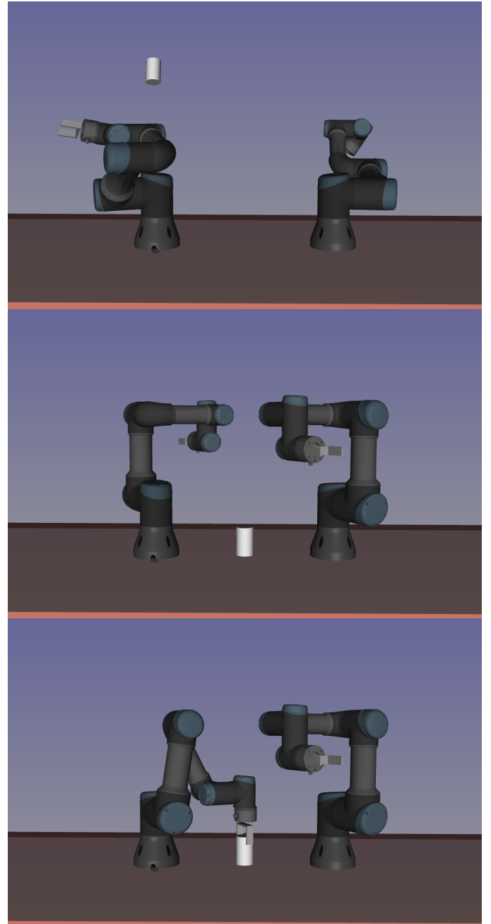
Fig. 3. Example of extension along a transition of the constraint graph. Top \mathbf{q}_{rand} , middle \mathbf{q}_{near} , bottom \mathbf{q}_{target} .
