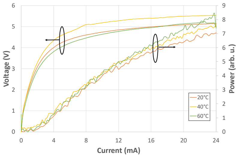
Figure 6. L-I-V characteristics of 50μm-wide-apertured VCSELs as a function of temperature
