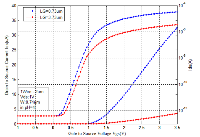
Fig3. In linear and semi-logarithmic scale the Si-nw-ISFFET I_{ds} ( V_{gs} ) consist of a single nanowire, different gate lengths ( 0.73\mu m and 3.73\mu m ) and the length of 2\mu m nanowire. ( V_{DS} = 1V )
