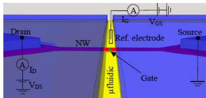
Fig1. Schematic view of Si-nw-ChemFET sensor
