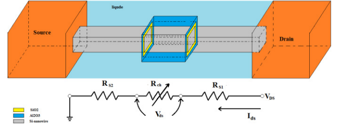
Fig2: parasitic series resistance of nanowire
