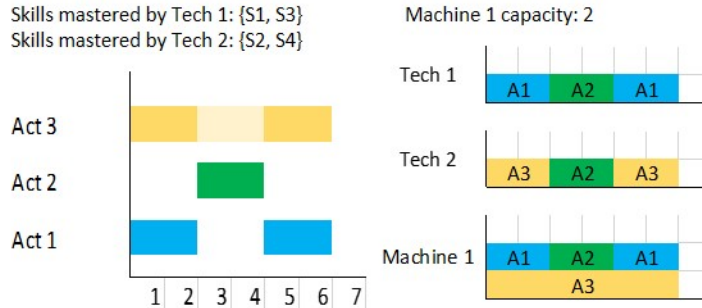
Fig. 1. Example of an MSPSP-PP instance.
