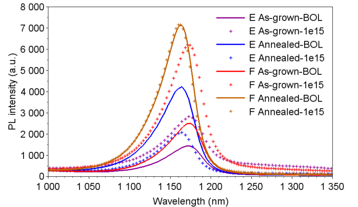
Fig. 8. PL spectra of samples before and after 10^{15} \text{ cm}^{-2} 1 MeV electrons irradiation obtained at room temperature
